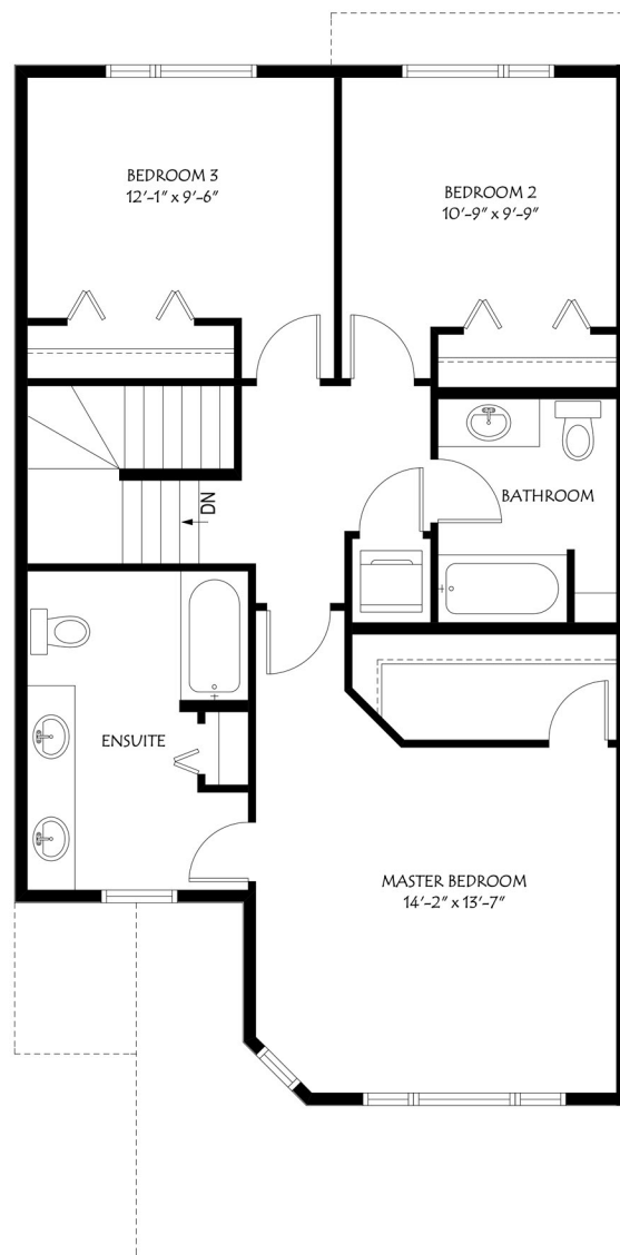
SECOND FLOOR 916 SQFT
